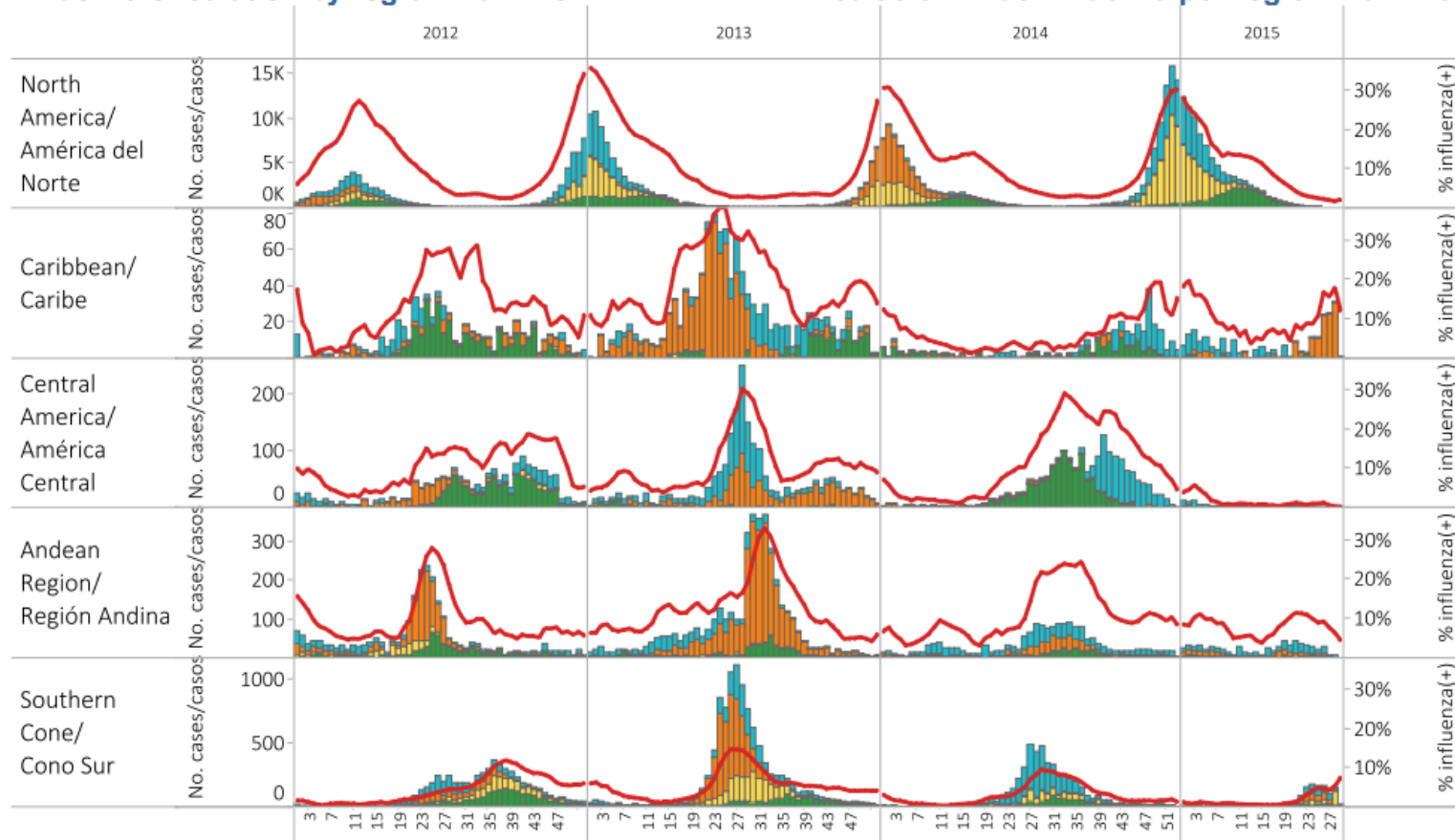
Influenza circulation by region. 2012-15
